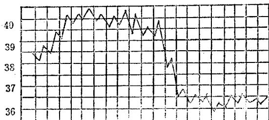
图 2-1 稽留热
