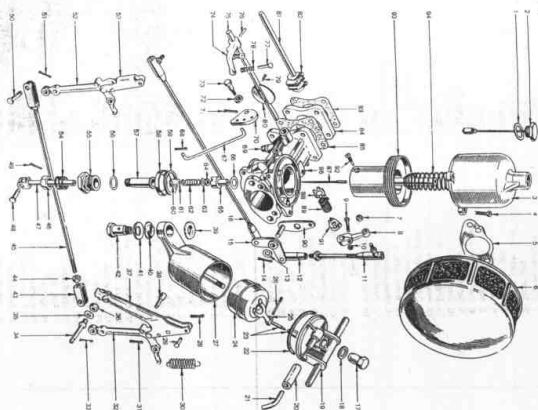
Carburetor
