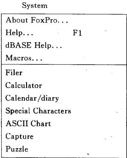
图2.1 System 菜单
