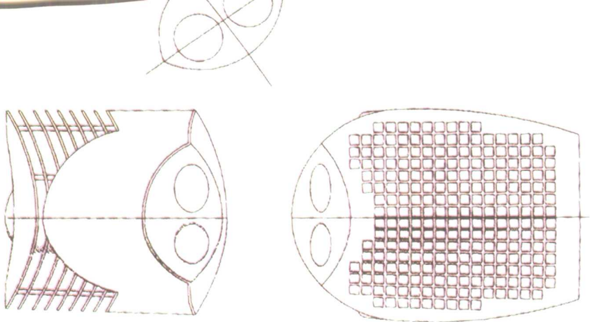
Fan Heater PTC ceramic Mod. ATL-430 1500/2000w 2736pcs/542pcs
