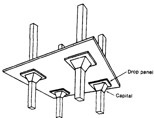
(c) Flat slab
