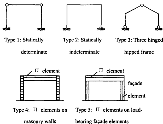
Fig. 1-3 Types of structural frames
