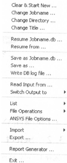
图 1-7 File 菜单
