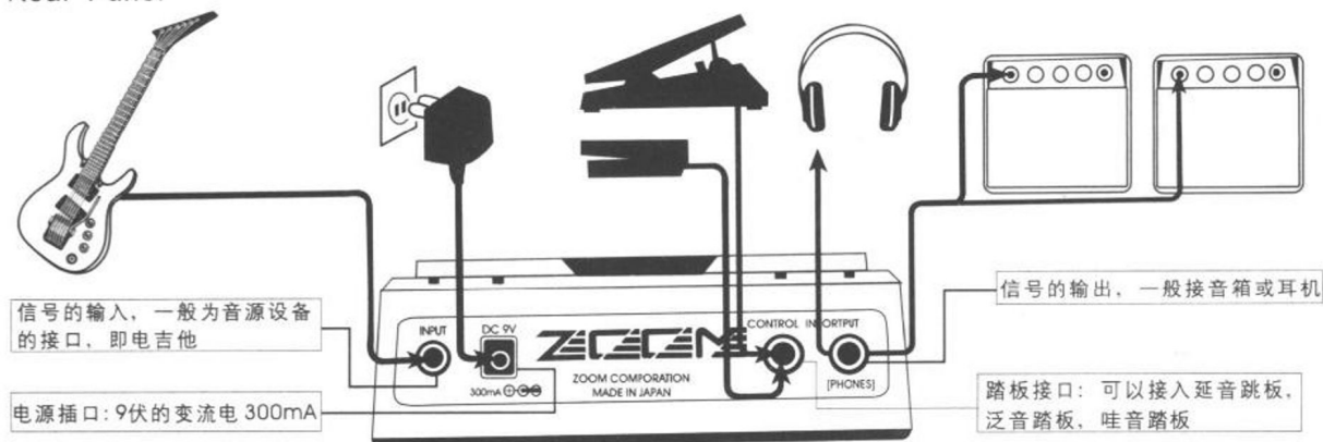
Rear Panel
