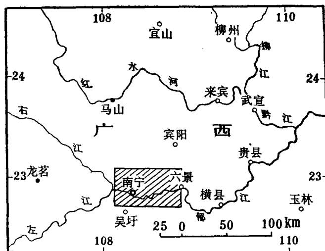
插图 1 广西南部勘察位置简图 (Outline map showing the location of the area of southern Guangxi studied in this paper.)
