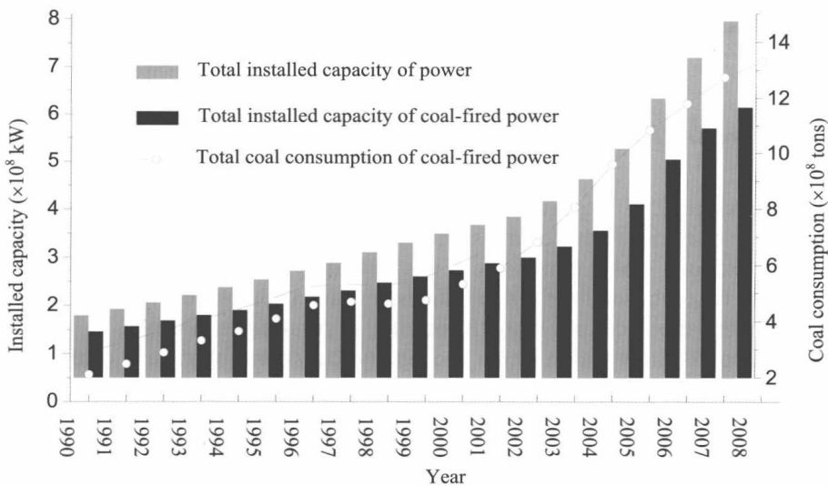
Fig. 1.2 Capacity and coal consumption of electric power generation in China from 1990 to 2008
