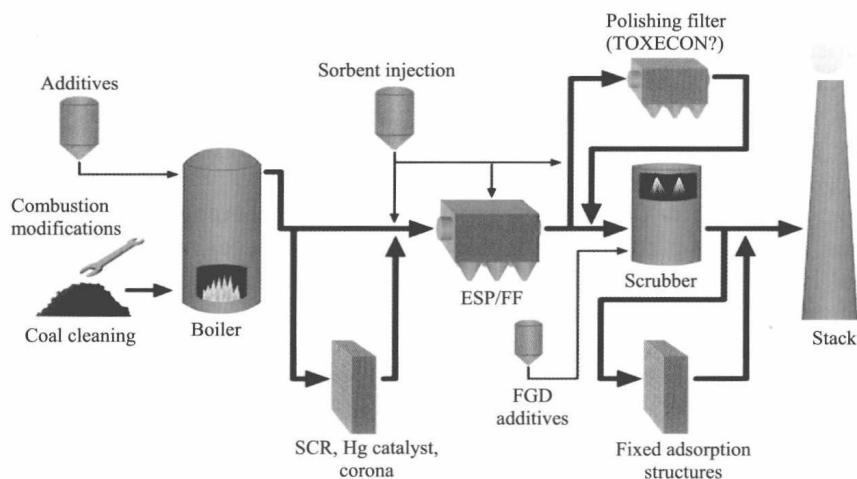
Fig. 1.3 Mercury pollution control technical methods for coal-fired power plants
