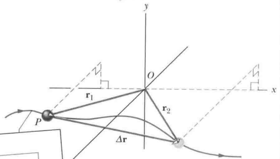
Sample Problem 4-1. The displacement \Delta\mathbf{r} = d of \mathbf{r}_1 to the head of \mathbf{r}_2 .
