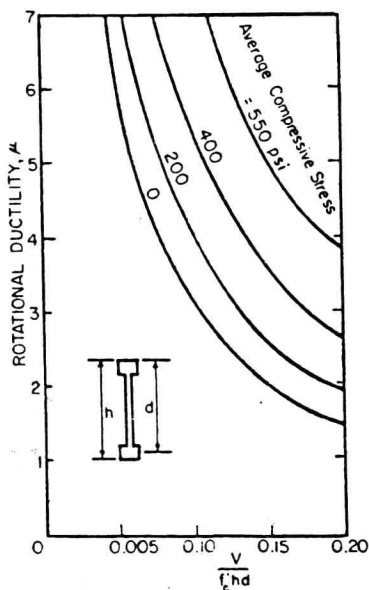
Fig. 8 Rotational Ductility Ratio, \mu_r
