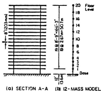
Fig. 1 Twenty-Story Isolated Structural Wall Model
