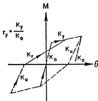
Fig. 2 Hysteretic Loop of Decreasing-Stiffness Model
