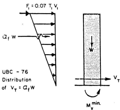
Fig. 7 Distribution of Lateral Forces Along Height of Isolated Structural Walls
