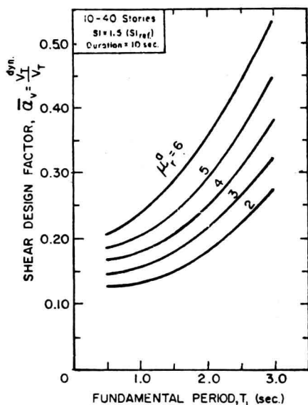
Fig. 6 Shear Design Factor, \bar{\alpha}_v
