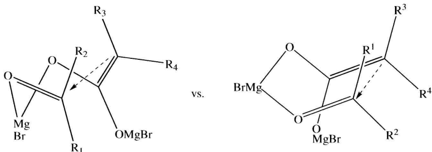
TS A: chairlike transition structure
