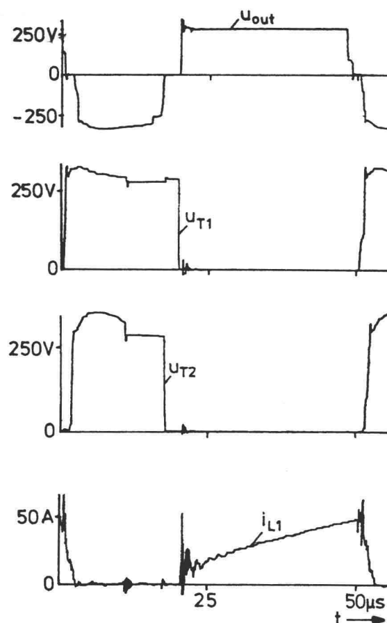
Fig. 6: Waveforms of a switching cycle at 20kHz
