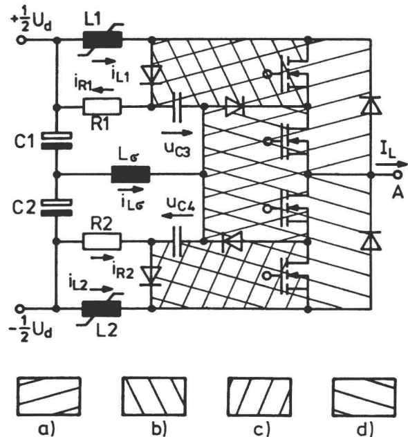
Fig. 2: The four critical commutation loops of the inverter leg marked by different hatching patterns a) ... d)
