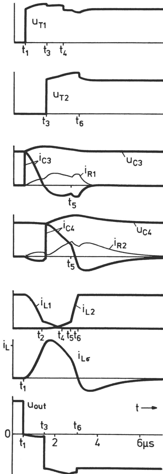
Fig. 3 (right): Computed waveforms of the commutation of a positive load current from T1 to D2
