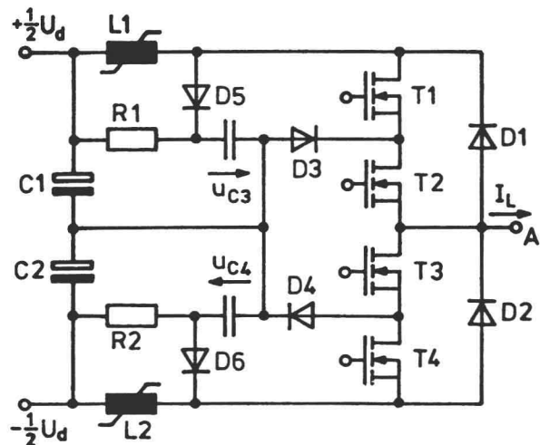
Fig. 1: Circuit diagram of one leg of a high-voltage MOSFET inverter
