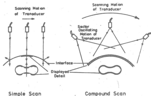
Fig. 1-2. Comparison of simple and compound scan.
