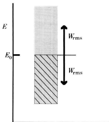
Figure 1. Electron energy levels of a system with a large number of atoms, spread into a band of root-mean-square width W_{\text{rms}} . For a half-filled band the shaded states are occupied by electrons.
