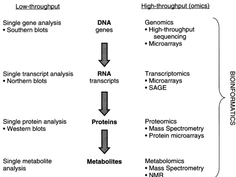
Figure 1.1 The relationship of the central dogma of molecular biology to omics technologies. The central dogma involves the organization and flow of information from DNA to RNA to proteins and the resultant metabolites. Developing an understanding of the interrelations of these levels is the focus of biological research. Omic technologies represent high-throughput and expansive approaches to the study of each of these levels. Bioinformatics is a key component to the interpretation and integration of the complex data-sets generated by omic technologies.
