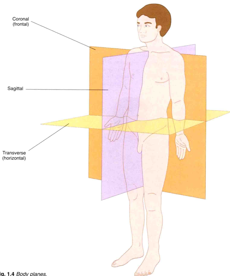
Fig. 1.4 Body planes.
