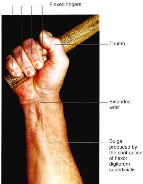
Fig. 2.3 Power grip.
