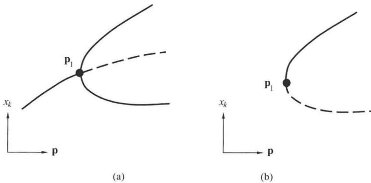
Figure 1.1 Bifurcation types: (a) period-doubling and (b) saddle-node
