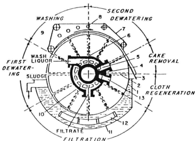
FIGURE 1.3. Diagrammatic cross section of rotary-drum vacuum filter: (1) drum, (2) connecting pipe, (3) scraper, (4) automatic valve, (5, 13) chambers of automatic valve connected with a source of compressed air, (6, 10) chambers of automatic valve connected with a source of vacuum, (7) endless belt, (8) wash header, (9) guiding roll, (11) tank for suspension, and (12) stirring device.
