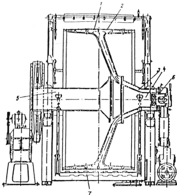
FIGURE 1.2. Longitudinal section of a rotary-drum vacuum filter with an external filtration surface: (1) drum, (2) compartment, (3) connecting pipe, (4) hollow trunion, (5) shaft, (6) automatic valve, and (7) stirring surface.
