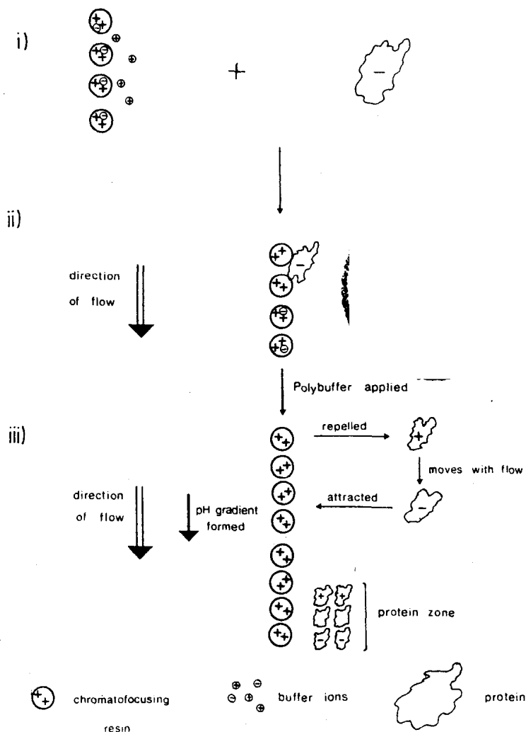
Figure 1.6: Principles of chromatofocusing chromatography
