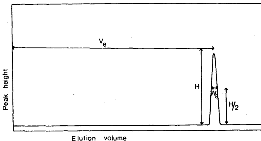
Figure 1.4: Calculation of theoretical plates for a chromatography column
