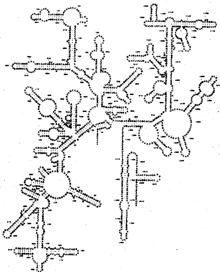
FIG. 3. Secondary structure of 16-S rRNA (26).
