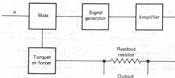
Fig. 7. Force-balance hinged-pendulum accelerometer. a = response to an acceleration.
