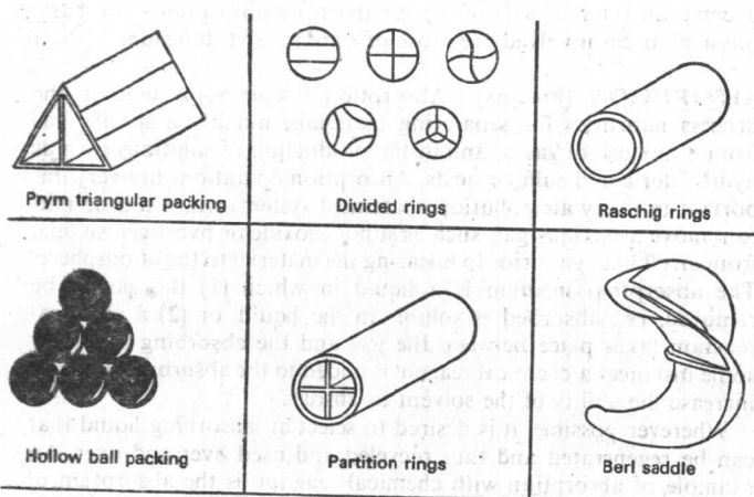
Fig. 2. Types of packing used in absorption towers.
