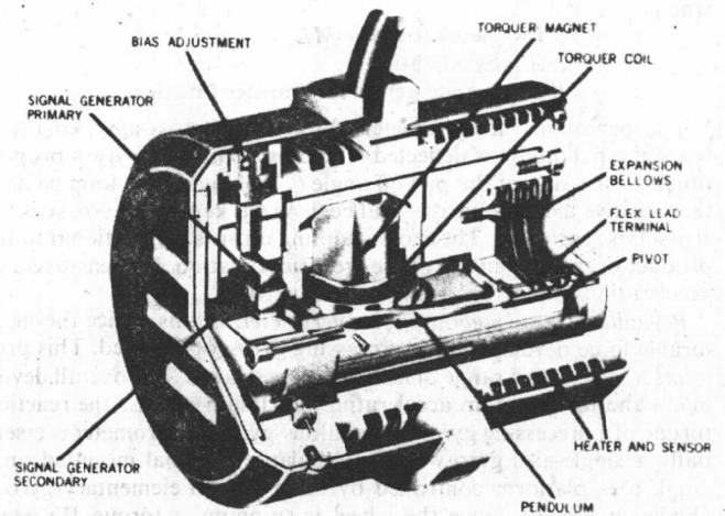
Fig. 8. Force balance accelerometer. No external amplifier. (Honeywell)
