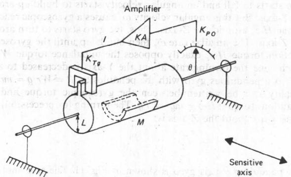
Fig. 9. Operating principle of pendulous accelerometer.
