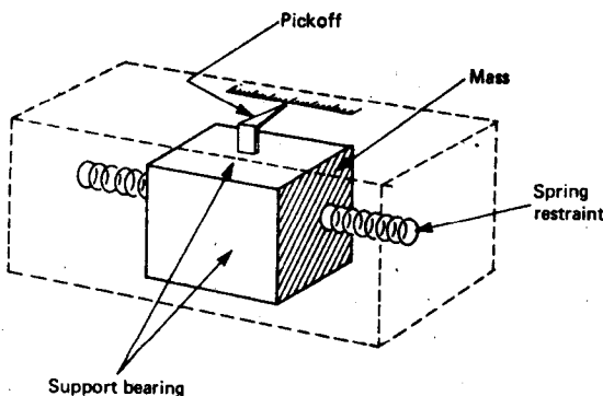
Fig. 1. Accelerometer based on a spring-restrained mass.
