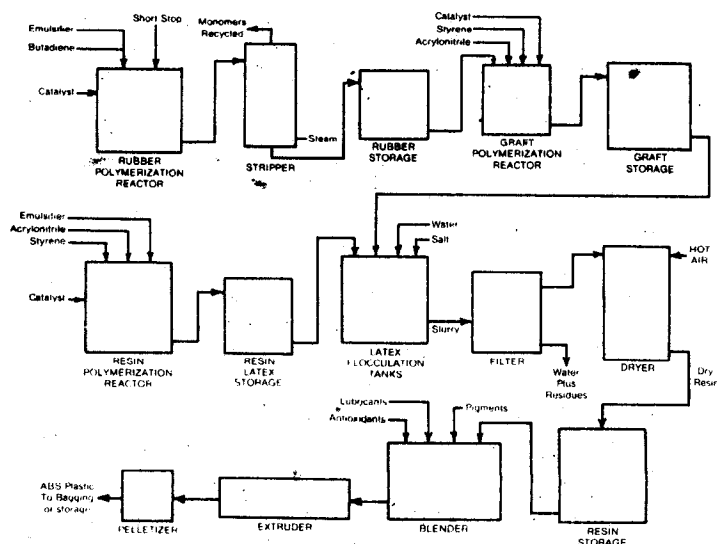
ABS manufacturing process. (Marlon Division, Borg-Warner Corporation)
