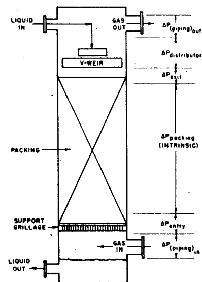
Fig. 1. Section of representative packed absorption tower.
