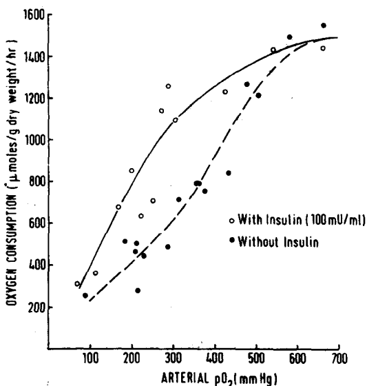
FIG. 1, 2. The relationship between arterial oxygen tension and oxygen consumption in the presence and absence of insulin. The data were obtained from 15 hearts.
