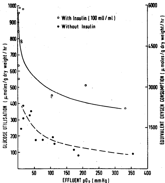
FIG. 1, 4. The relationship between the oxygen tension of the coronary effluent and glucose utilization and equivalent oxygen consumption in the presence and absence of insulin. The data were obtained from 15 hearts.
