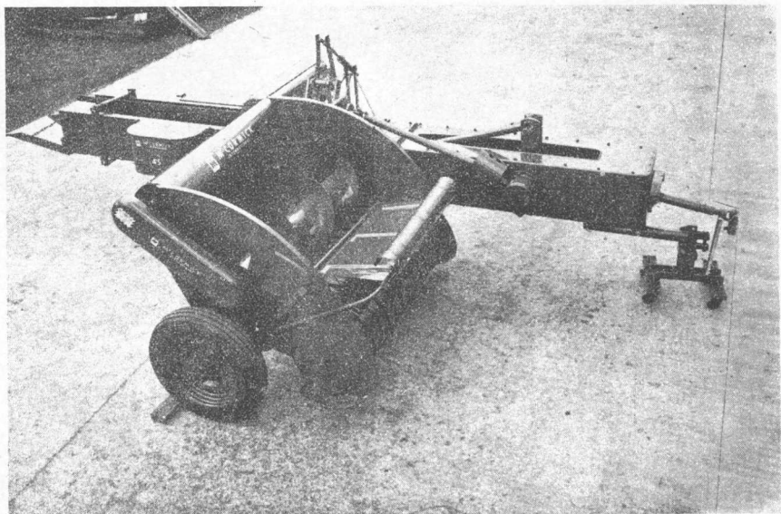
14. No. "45" Pick-up Baler (International Harvester Co. Ltd., London)
