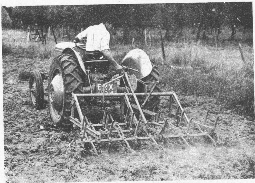
6. Combined Arable and Pitch Pole Harrow fitted to three-point linkage of the Ferguson Tractor
