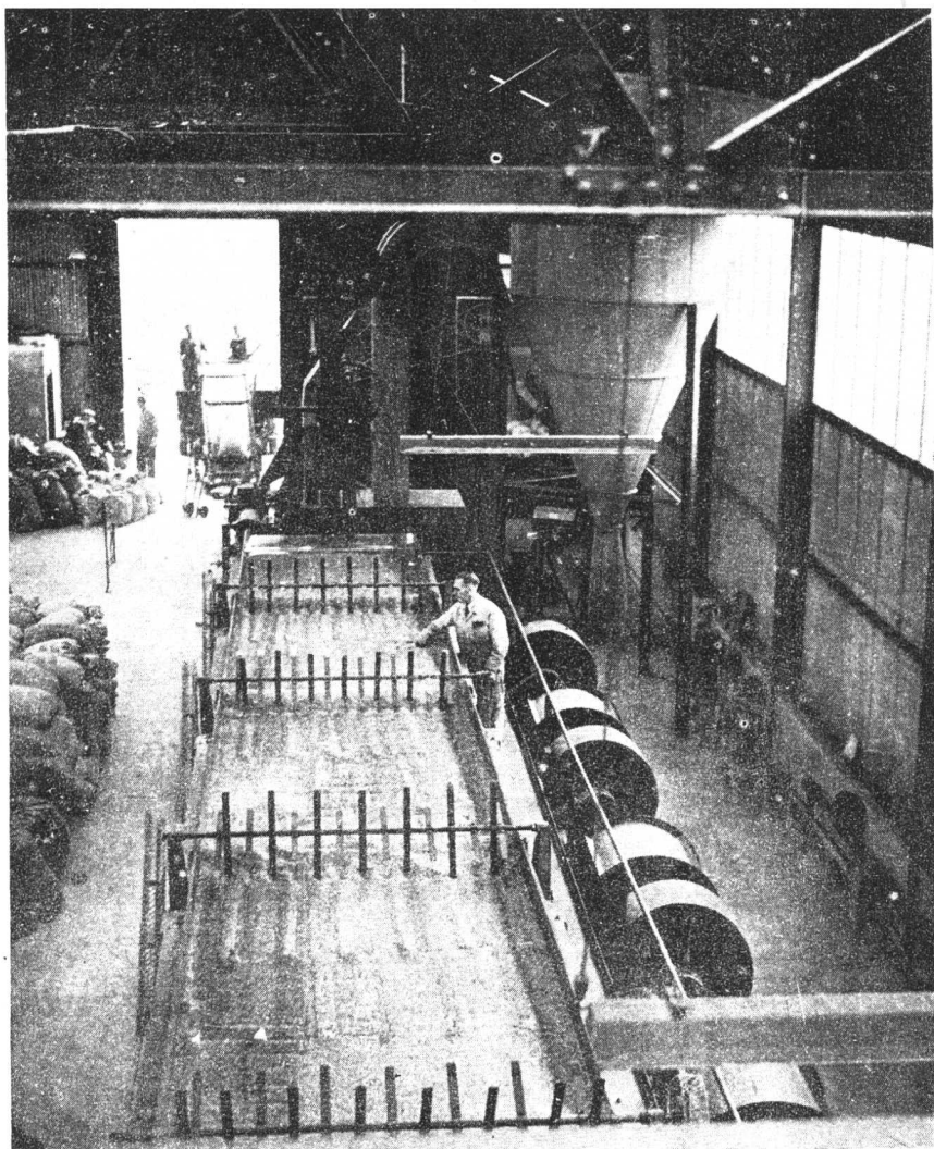
16. A Grain-drying Plant. The grain is delivered from a storage container to the heating trays along a chute, and is then propelled along the trays to a cleaning machine, seen in the background, from which it is run into sacks
