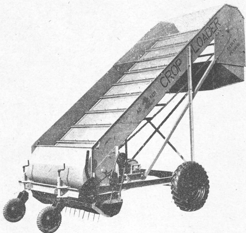
13. "Ad Rem" Crop Loader
