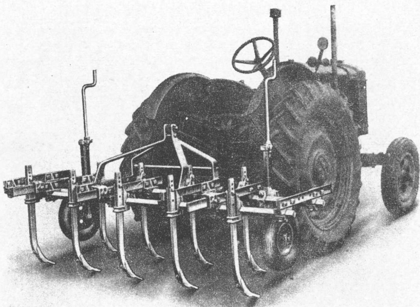
5. Ransomes Toolbar Frame
