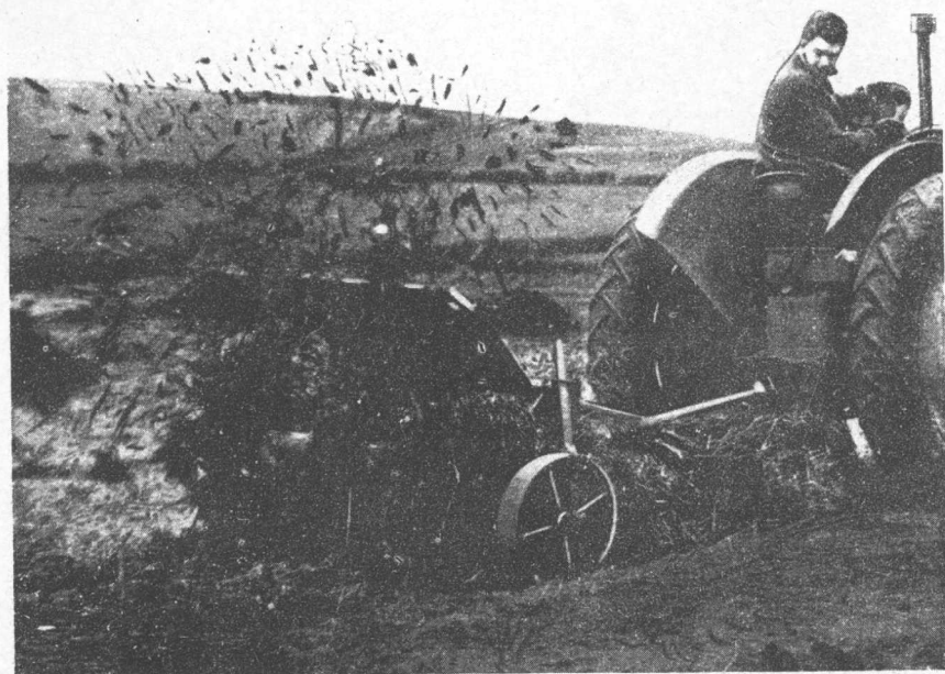
10. Wild-Thwaites Muck Spreader
