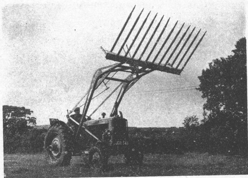
12. Horn-draulic Crop Loader
