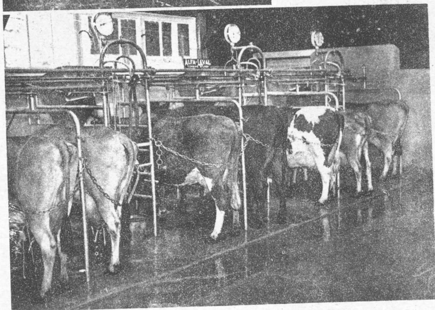
18. Alfa-Laval Combine Recorder Milking Machine (Alfa-Laval Co. Ltd., Brentford)
