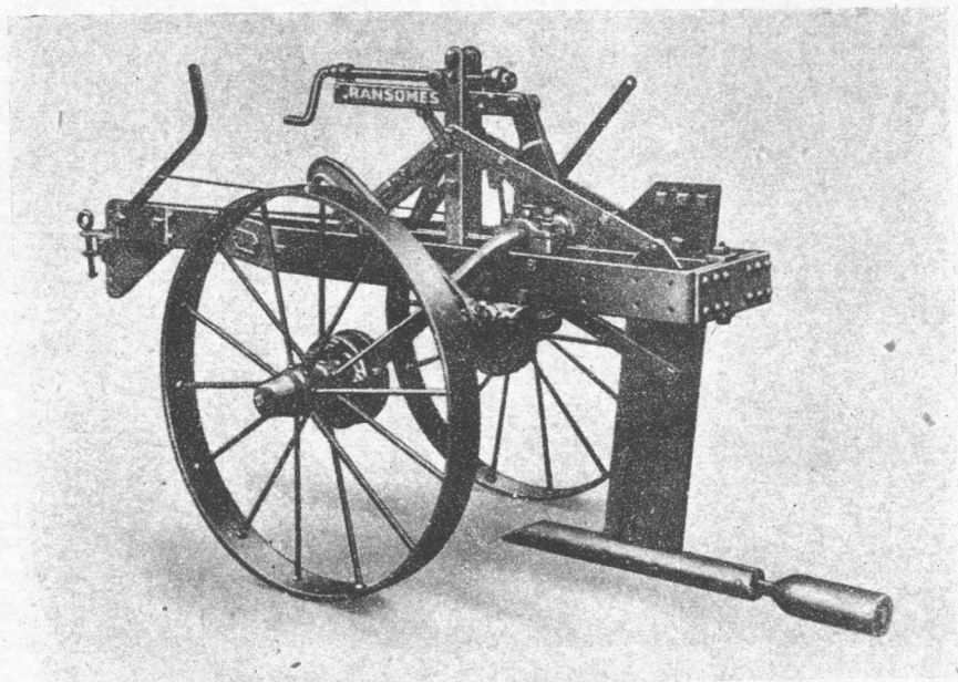
1. Ransomes Mole Drainer
