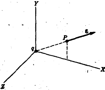
Fig. 1-1. Electric field of a charge at rest.
