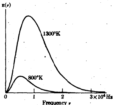
Fig. 1-4. Monochromatic energy density of blackbody radiation at different temperatures as a function of the frequency.
