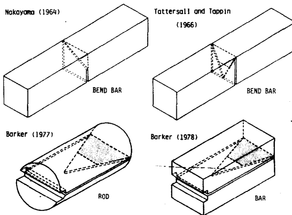
FIG. 1—Various chevron-notched fracture specimen configurations.
