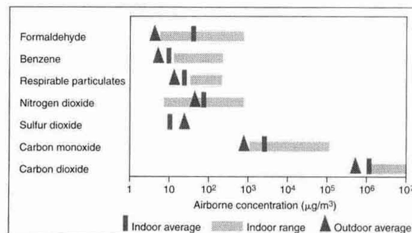
Figure 1.11 Indoor and outdoor concentrations of common pollutants
