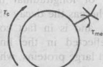
Fig. A4. Diagrammatic representation of a methyl group anisotropically rotating on a globular macromolecule. The correlation times are denoted by \tau_{me} and \tau_c respectively.
