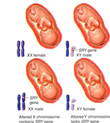
Figure 6.23 Illegitimate recombination may produce an XY female or an XX male. The SRY gene, normally located on the Y chromosome, dictates male development; in the absence of SRY , an embryo develops as a female. Rare, illegitimate recombination between the X and Y chromosome can create a Y chromosome without SRY and an X chromosome with SRY . Fertilization with gametes containing these unusual chromosomes will produce XY females or XX males.
