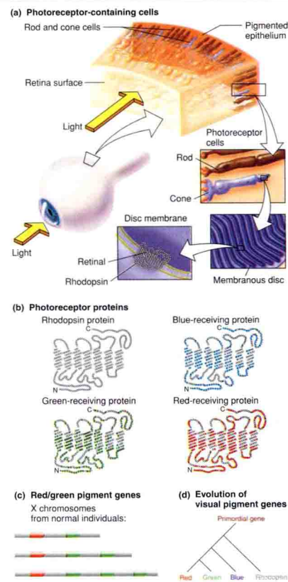
Figure 7.28 The cellular and molecular basis of vision. (a) Rod and cone cells in the retina carry membrane-bound photoreceptors. (b) The photoreceptor in rod cells is rhodopsin. The blue-, green-, and red-receiving proteins in cone cells are related to rhodopsin. (c) One red photoreceptor gene and one to three green photoreceptor genes are clustered on the X chromosome. (d) The genes for rhodopsin and the three color receptors probably evolved from a primordial photoreceptor gene through three gene duplication events followed by divergence of the duplicated copies.
