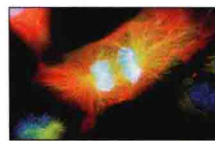
(d) Anaphase: (1) Centromeres divide; (2) the now separated sister chromatids move to opposite poles.
