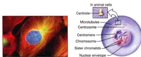
(a) Prophase: (1) Chromosomes condense and become visible; (2) centrosomes move apart toward opposite poles and generate new microtubules; (3) nucleoli begin to disappear.
