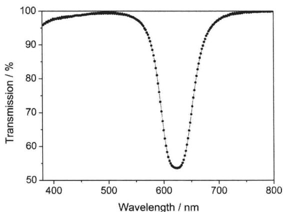
Figure 1.2 Transmission spectrum of a cholesteric liquid crystal.
