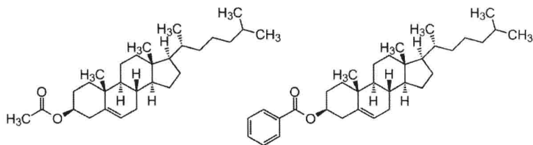
Figure 1.3 Molecular structures of cholesteryl acetate (left) and cholesteryl benzoate (right).
