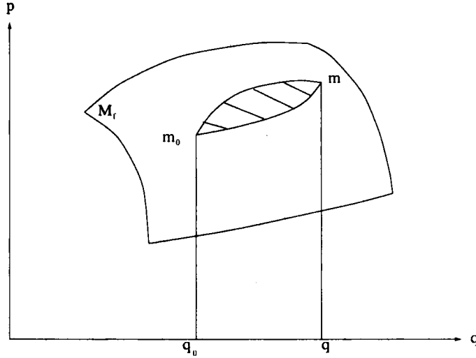
Fig. 2.1. A leaf M_f on phase space
