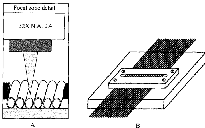
Figure 1.3 The exploded schematic view of focal zone (A) and the capillary array holder (B) of the laser-excited, confocal fluorescence capillary array scanner. From Huang X H C, Quesada M A, and Mathies R A. Capillary array electrophoresis using laser-excited confocal fluorescence detection. Anal Chem, 1992, 64(8): 967-972.
