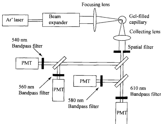
Figure 1. 2 Optical system employed for multiple wavelength fluorescence detection in capillary electrophoresis of DNA. From Luckey J A, Drossman H, Kostichka A J, et al. High-speed DNA sequencing by capillary electrophoresis. Nucleic Acids Res, 1990,18(15): 4417-4421.
