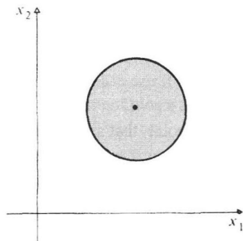
Fig. 1.1. The distance function d(x, y) defines a neighborhood in R^2 which is the interior of the disc bounded by the circle of radius r . The circle itself is not part of this neighborhood.
