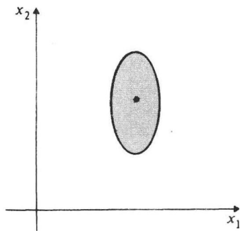
Fig. 1.3. The distance function d'(x, y) = [4(x_1 - y_1)^2 + (x_2 - y_2)^2]^{1/2} defines a neighborhood in R^2 which is the interior of the disc bounded by the ellipse 4(x_1 - y_1)^2 + (x_2 - y_2)^2 = r^2 . As in figure 1.1, the ellipse itself is not in the neighborhood.
