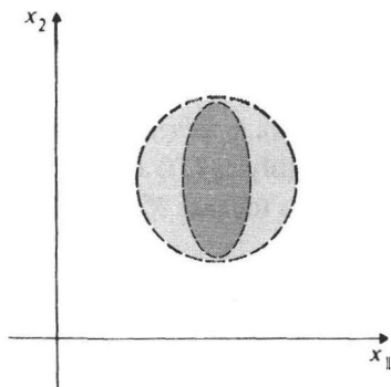
Fig. 1.4. In R^2 a d -neighborhood of radius \epsilon (bounded by the circle) entirely contains a d' -neighborhood of radius \delta (bounded by the ellipse defined in figure 1.3) if \delta < \epsilon . If \delta > 2\epsilon the inclusion is reversed.
