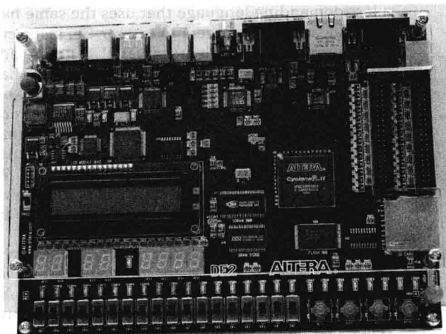
FIGURE P-2 Altera's DE2 development board.
