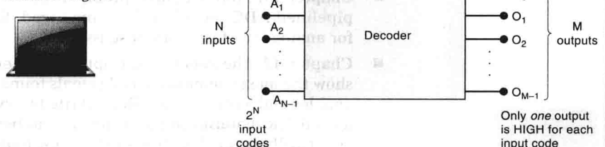
FIGURE 9-1 General decoder diagram.
