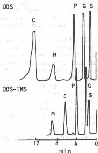
Fig. 1. Comparison of ODS silica (upper) with ODS-TMS silica packing (lower; TMS = trimethylsilyl) for separating paracetamol and its metabolites ([5], by permission).
