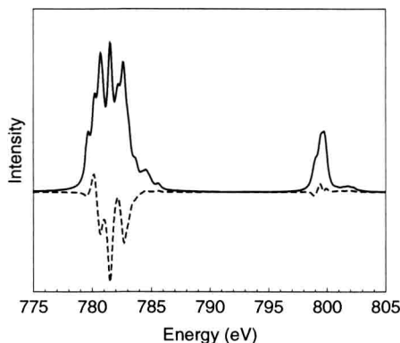
Figure 1.1 The isotropic (solid) and circular dichroic (dashed) spectra of divalent cobalt in an octahedral crystal field.
