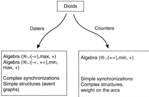
Figure 1.4. Daters and counters
