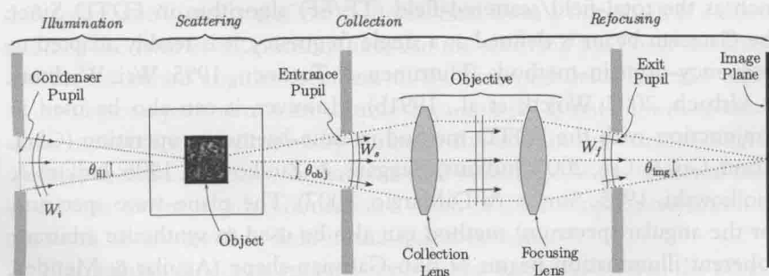
Figure 1 The four subcomponents of an optical imaging system: illumination, scattering, collection, and refocusing.
