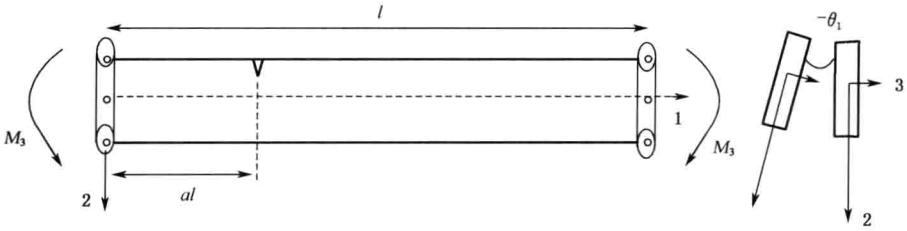
Figure 1 Lateral-torsional buckling of a cracked beam under uniform bending moment
