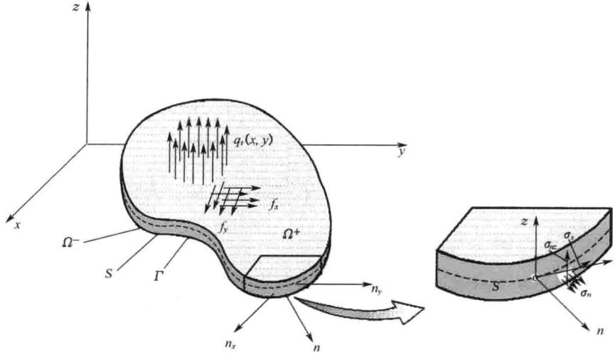
Figure 1 Geometry of a plate loaded with forces.
