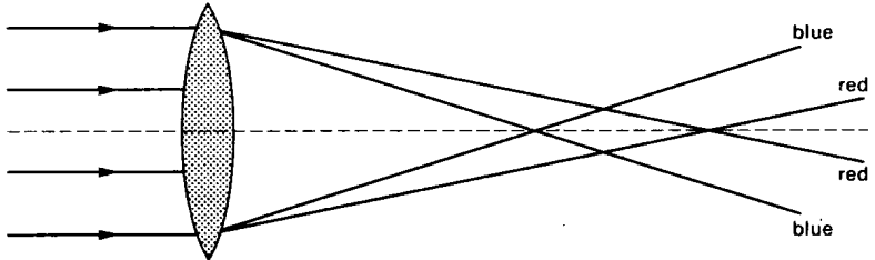
chromatic aberration
