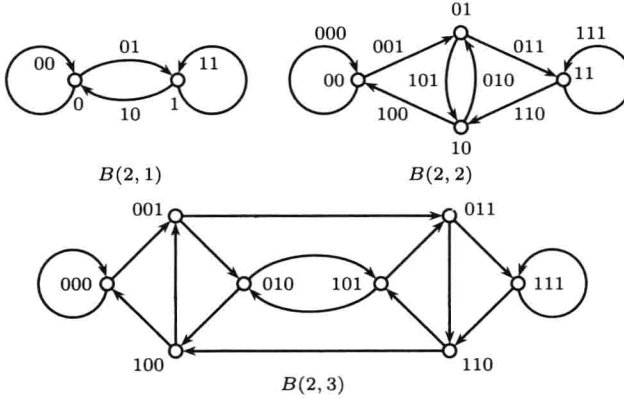
Figure 1.5 De Bruin digraphs B(2, 1) , B(2, 2) and B(2, 3)
