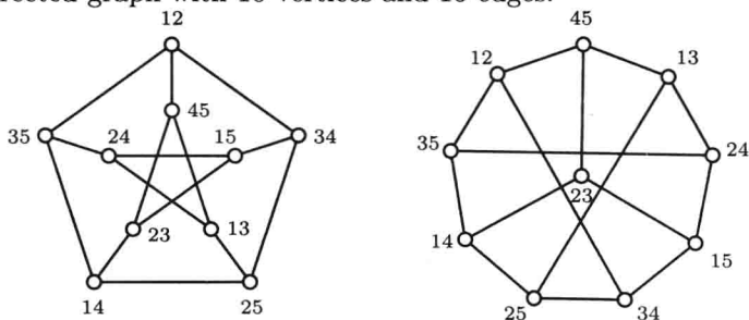
Figure 1.3 Two drawings of the J(5, 2, 0) -graph
