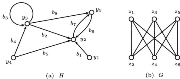
Figure 1.2 Graphical representations of graphs H and G
