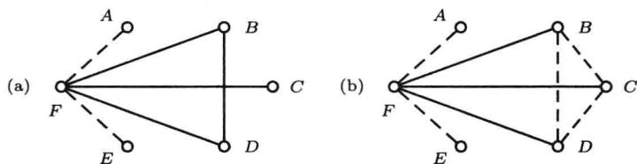
Figure 1.8 Illustrations in the proof of Example 1.1.8
