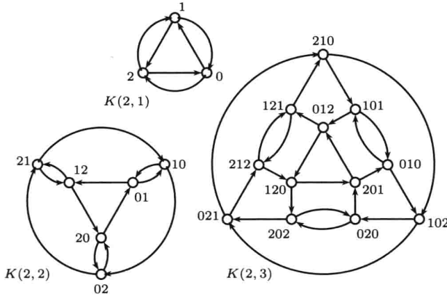
Figure 1.6 Kautz digraphs K(2, 1) , K(2, 2) and K(2, 3)
