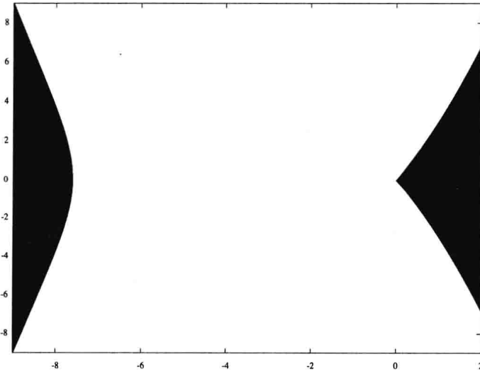
Figure 1.2. Numerically computed planar section through (Q, 0)
