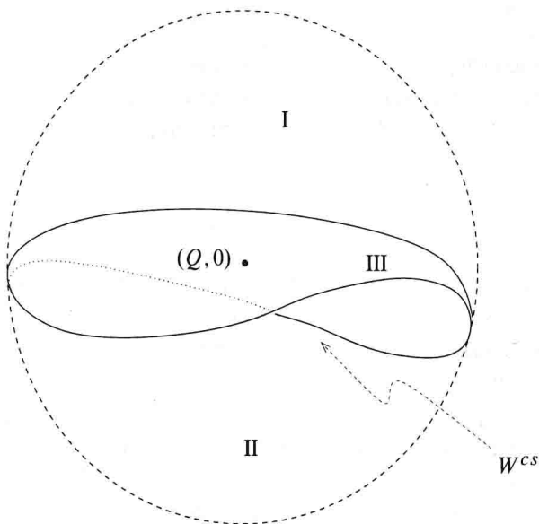
Figure 1.1. The forward trichotomy near (Q, 0)
