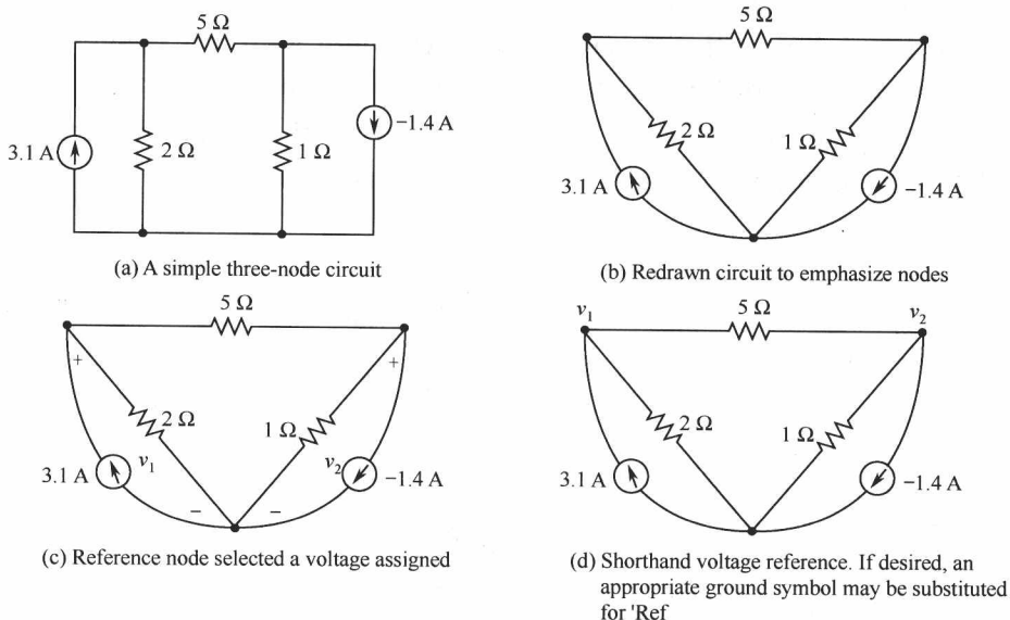
Fig. 1-A-4 The mechanics of node analysis.
