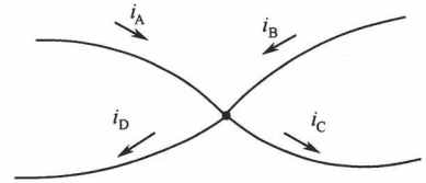
Fig. 1-A-2 Example node to illustrate the application of Kirchhoff's current law.
