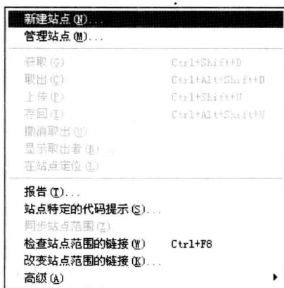
图 1-6 “站点”菜单
