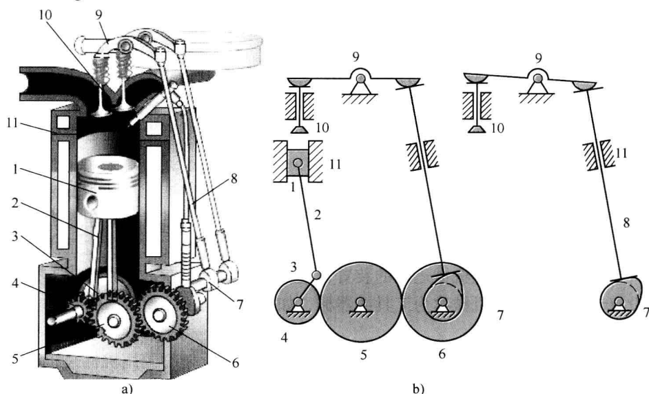
Fig. 1-1 Internal combustion engine and scheme (内燃机及其机构简图)
