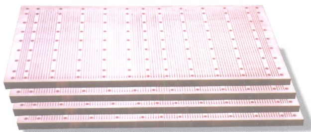
▲ 连续铸钢结晶器铜板（镀镍铁、镍钴） Copperplates with Continuous steel-casting crystallization.(nickel-coated iron and cobalt)
