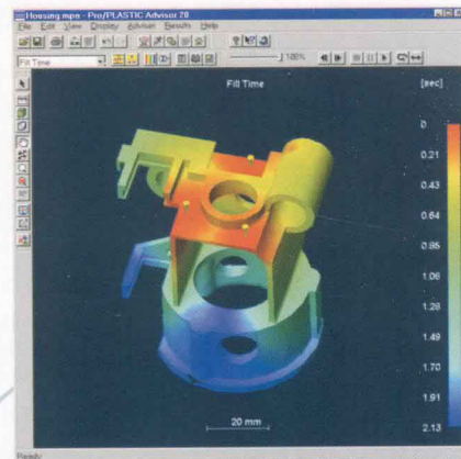
Mould Flow Analysis
