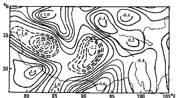
Fig. 3. Distribution of the vertically averaged "vertical velocity" \omega at 1800 h (Lhasa local time) in July 1979. Unit is in 10^{-3} hPa s ^{-1} . Adopted from Yang et al. (1992b)
