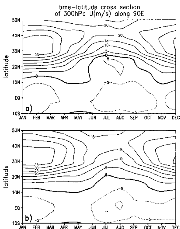
Fig. 9. The 10-year mean seasonal variation of the zonal wind component along 90^\circ\text{E} in the CON run (a), and in a parallel experiment (NSH) in which the surface sensible heating is removed from the plateau region where the absolute elevation is above 3 km (b). Unit is in \text{ms}^{-1}
