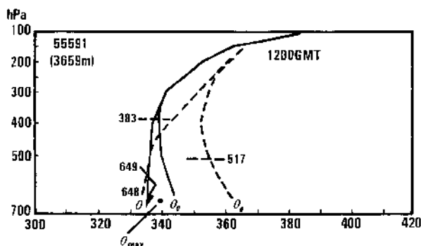
Fig. 1. Vertical profiles of 10-day mean potential temperature ( \theta ) and equivalent potential temperature ( \theta_e ) over Lhasa before (solid curves) and during (broken curves) the rainy season in 1979. Adopted from Luo and Yanai (1984)
