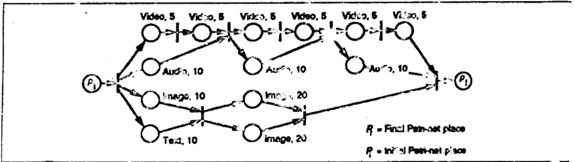
Figure 10. Temporal specification for a page.
