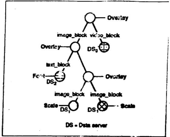
Figure 9. Spatial hierarchy for a page.
