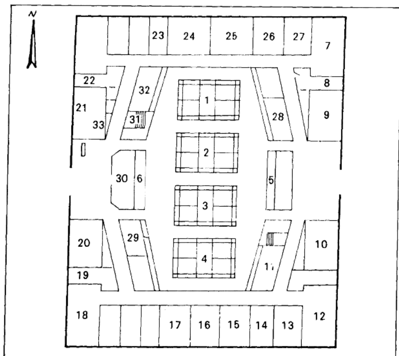
Plane Figure of the Competition Rooms of Huangpu Gymnasium
